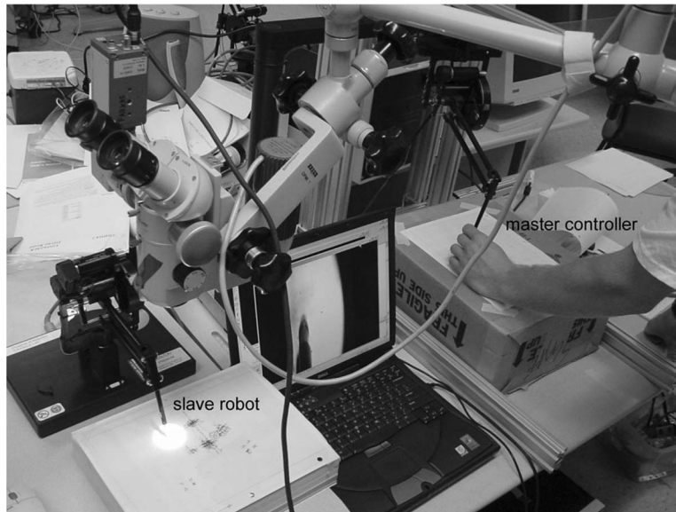
Fig. 11. Telepainter apparatus showing master and slave robots. The operator is manipulating the paintbrush handle held by the master (passive) robot while the slave robot is moving the paintbrush. The paper is white in this photo, though black paper was used during actual operation. The half-silvered mirror and flat-panel monitor over master controller are not shown.
